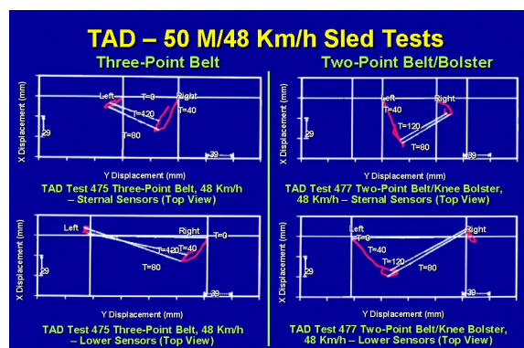
Figure 6 Comparison of TAD-50M Upper and Lower Thorax X-Y Deflection Crossplots for 3- Point and 2- Point Seat Belt Systems
