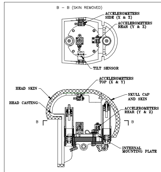
Figure 7 Thor Head Assembly
