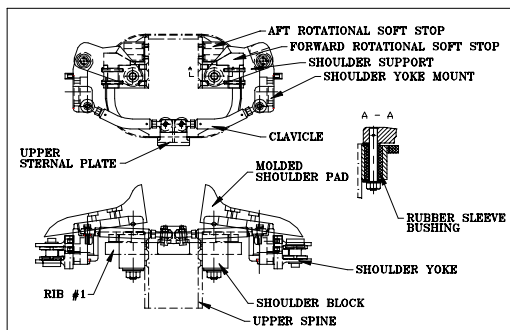
Figure 10 Thor Shoulder (as adapted from TAD-50M)
