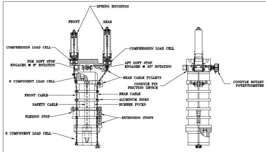
Figure 9 Thor Neck Design
