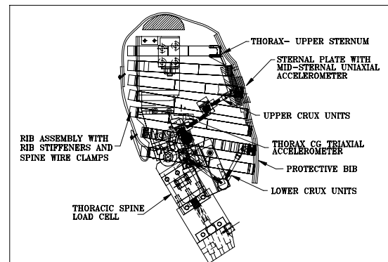
Figure 11 Side View of Thorax Assembly with Instrumentation
