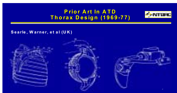
Figure 3 Ogle/MIRA and OPAT Thorax Design Concepts (1973-75)
