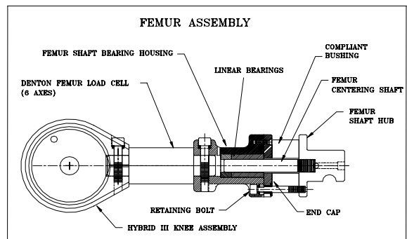
Figure 17 Thor Femur with Compliant Axial Element
