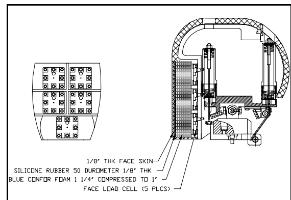
Figure 8 Thor Head/ Face Assembly
