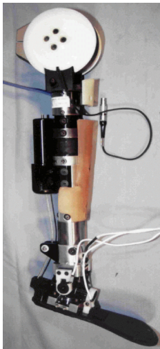
Figure 26 Thor-Lx/HIIIr Assembly (w/o flesh)
