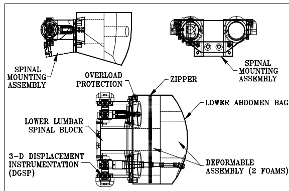
Figure 14 Lower Abdominal Assembly Showing Integral DGSP 3D Instrumentation
