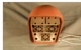
Figure 19 Thor ALPHA Face Load Cell Array (two cells not shown)
