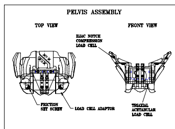
Figure 16 Pelvis Assembly Schematic
